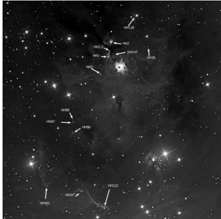
Observations of Herbig Haro Objects
