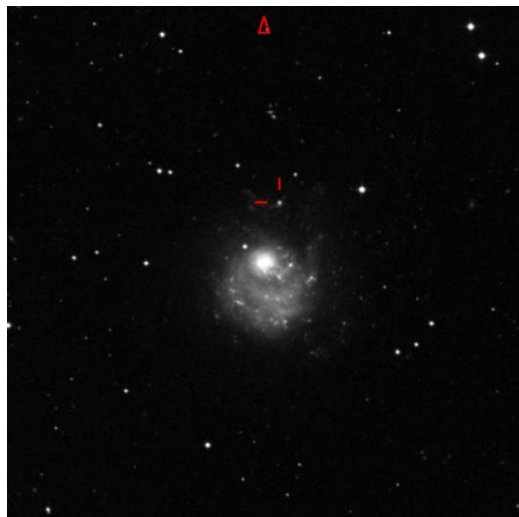
Observations of supernovae
