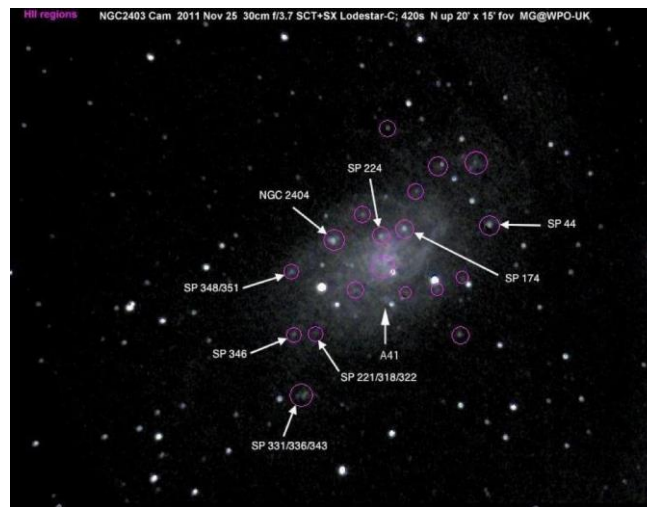
Observations of HII regions of NGC2403
